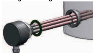
Mounting on welding sleeve
