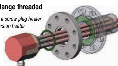
Mounting on flange threaded
